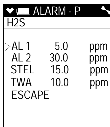
H2S
