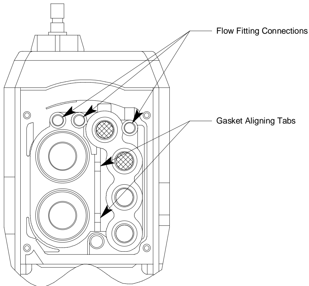
Figure 32: Sensor Gasket Seating
