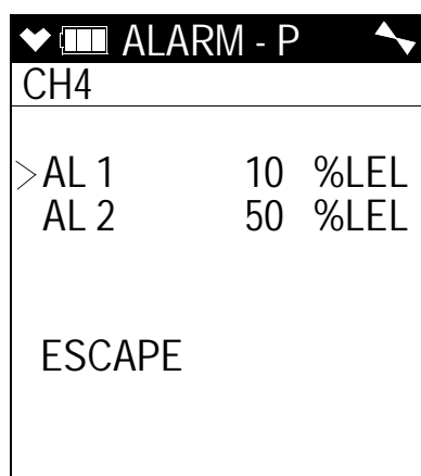
Catalytic LEL
