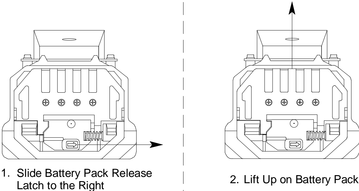
Figure 14: Releasing the Battery Pack
