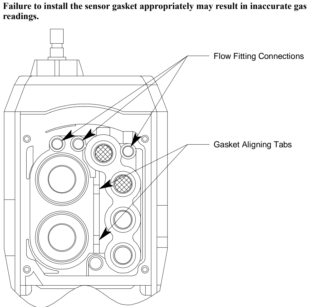
Figure 35: Sensor Gasket Seating
